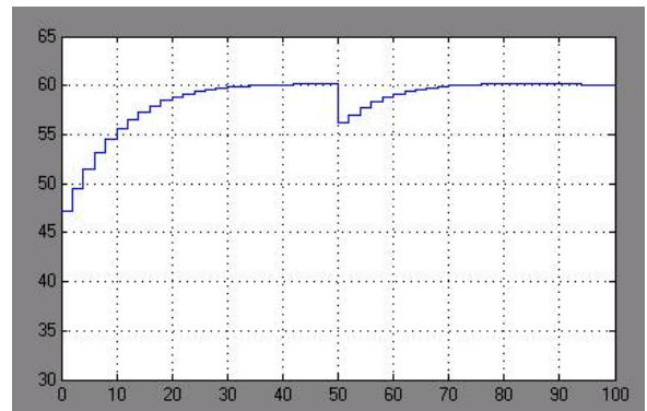
Fig. 5. FRC-6 - Reference tracking and disturbance's rejection
