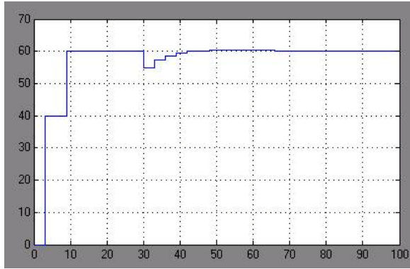
Fig. 1. FRC-1 - Reference tracking and disturbance rejection
