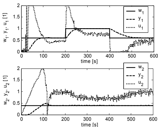
Fig. 8. Control courses without logical supervisor
