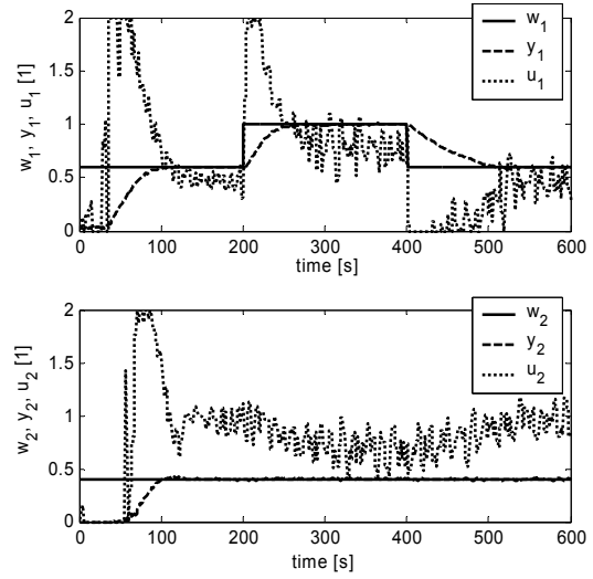
Fig. 6. Control courses without logical supervisor
