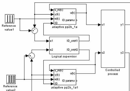
Fig 5. Simulink schema of control circuit
