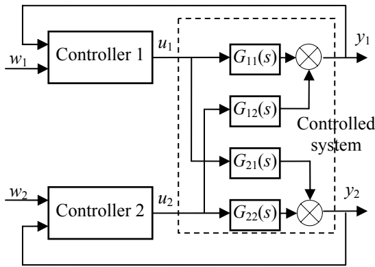
Fig. 1. Decentralized control of TITO system
