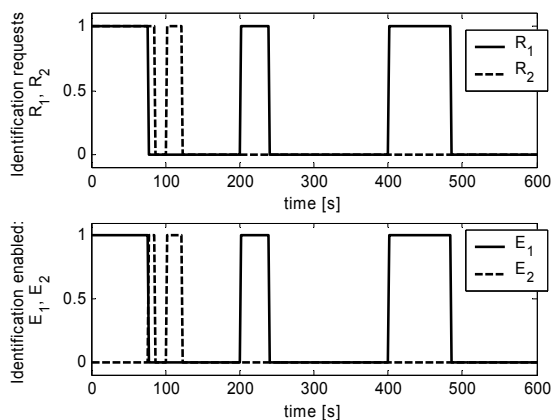
Fig. 10. Course of identification requests and identification enabled signals
