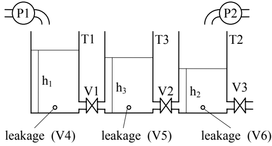
Fig. 4. Schema of three-tank system
