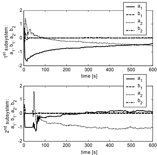
Fig. 7. Course of identification parameters during the control process without using logical supervisor
