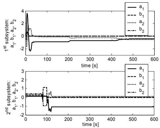
Fig. 9. Course of identification parameters during the control process with using logical supervisor
